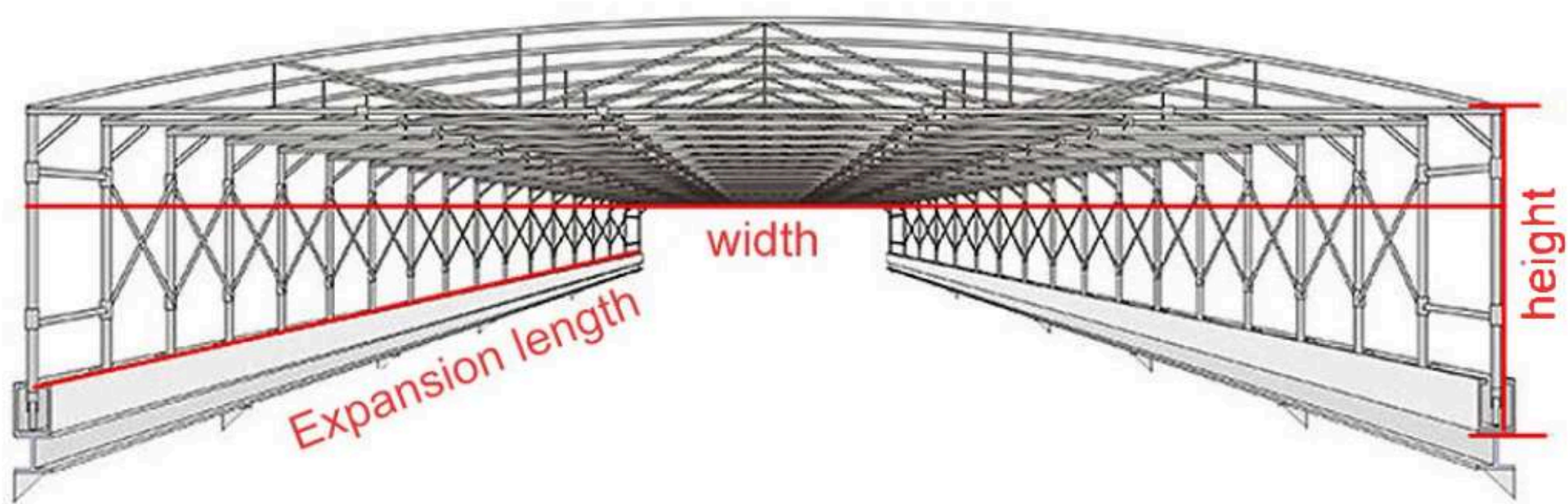
Structural Frame Combination Axonometric Drawing
